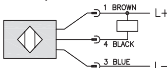
Diagram 2 NPN Output
