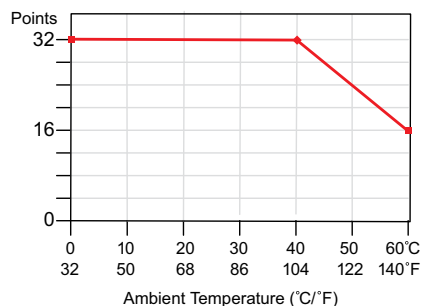
Derating Chart
