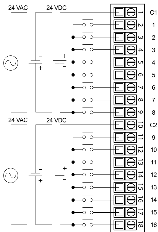
Equivalent Input Circuit
