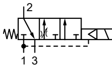
Soft Start/Dump Valve
