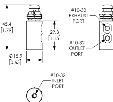
Part No. GVS-3C0F-PB-SS
