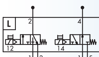
Diagram PAL-V2-53C
