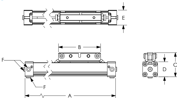
L-Series Rodless Pneumatic Cylinder Dimensions
