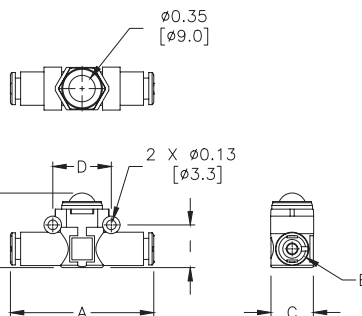
Silenced Exhaust
