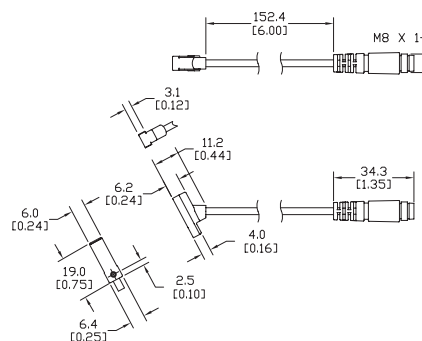
CPS9F-xx-F cable length tolerance w 1.5"
