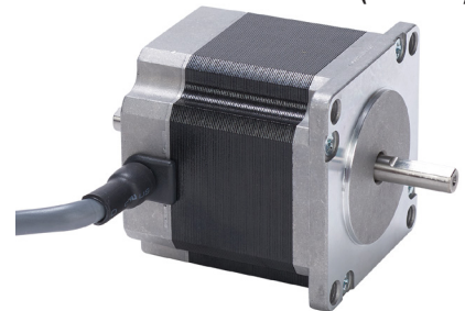
STP-MTRAC-xxxxxD (dual-shaft)
