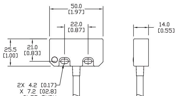
SWITCH
