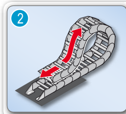
Installation option: Horizontal, gliding
