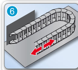
Installation option: Horizontal, side-mounted (rotated 90°), with support
