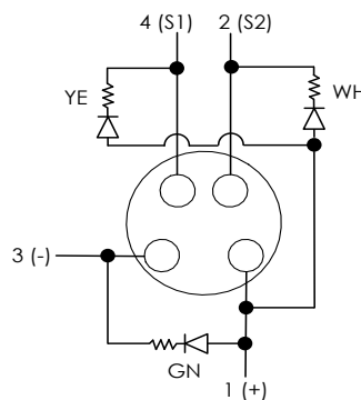
Diagram 6 (NPN field connection) 8000-84111-3580500 8000-88111-3950500
