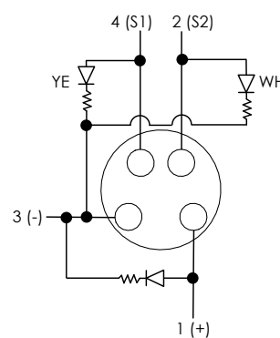
Diagram 4 (PNP field connection) 8000-84110-3580500 8000-88110-3950500 8000-84160-0000000
