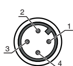
M12 connector
