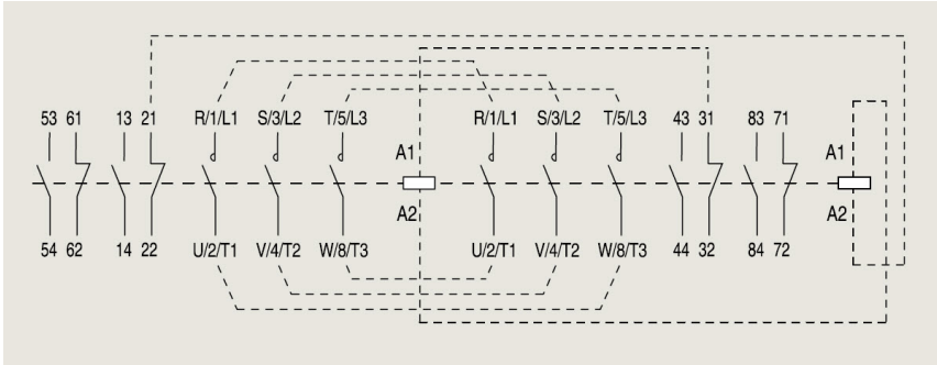
Typical circuit diagram for reversing contactor assembly
