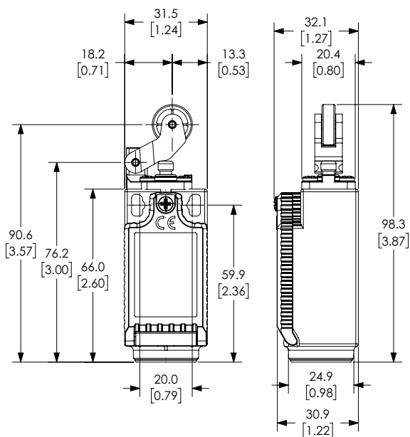
LSPS-171020 LSPS-171026
