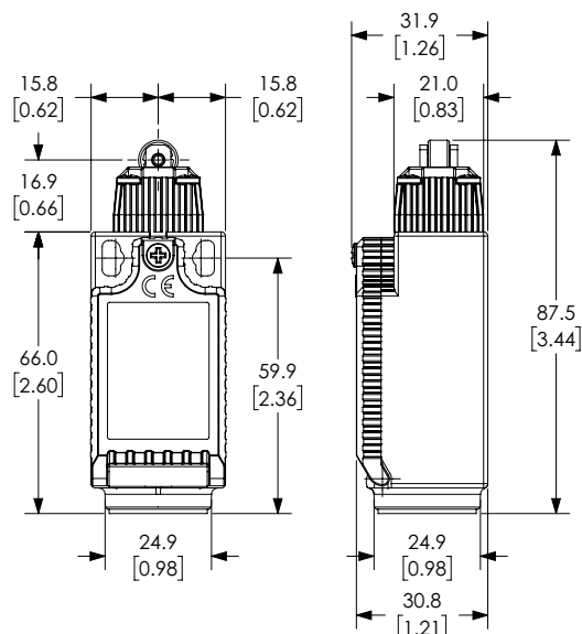
LSPS-171011 LSPS-171017
