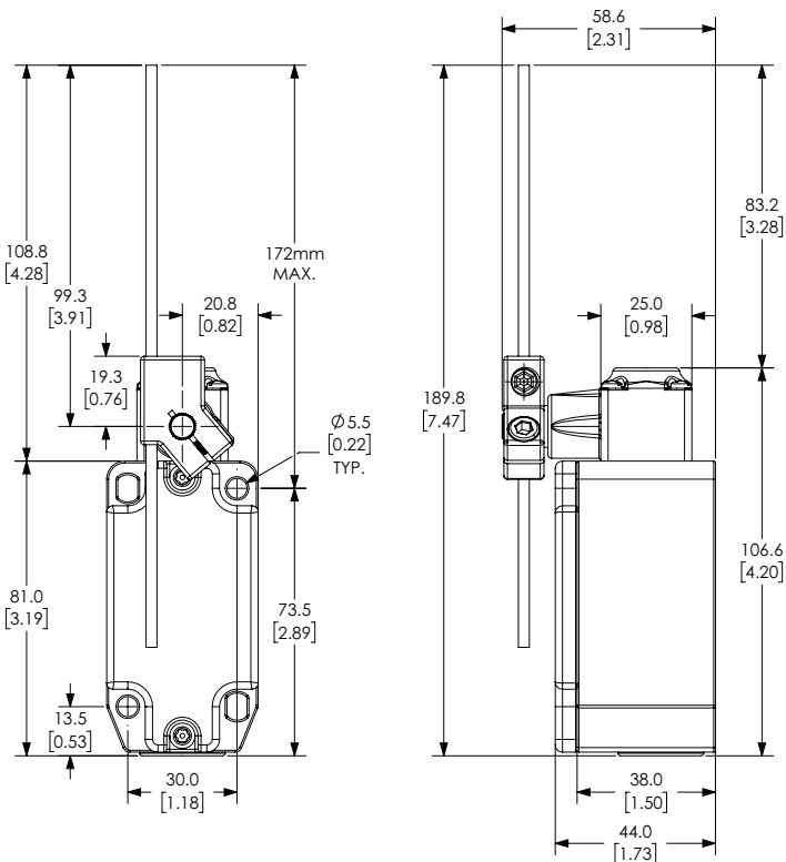
HLM-SS-175252 HLM-SS-175261
