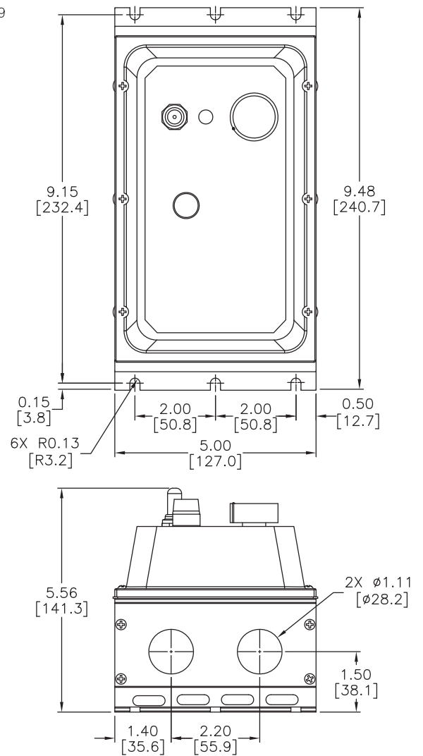
GSD4-240-10N4X Dimensions
