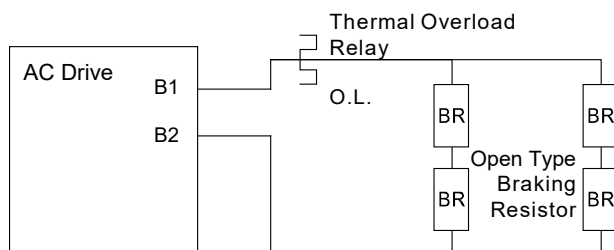
Diagram D (drive + 2 Series and 2 Parallel Resistors):
