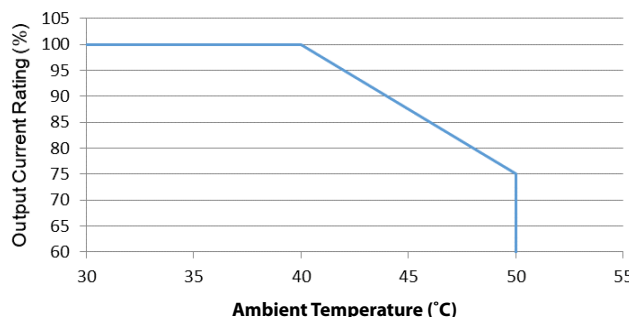
Ambient Temperature Derating of UL Type 4X / NEMA 4X / IP66
