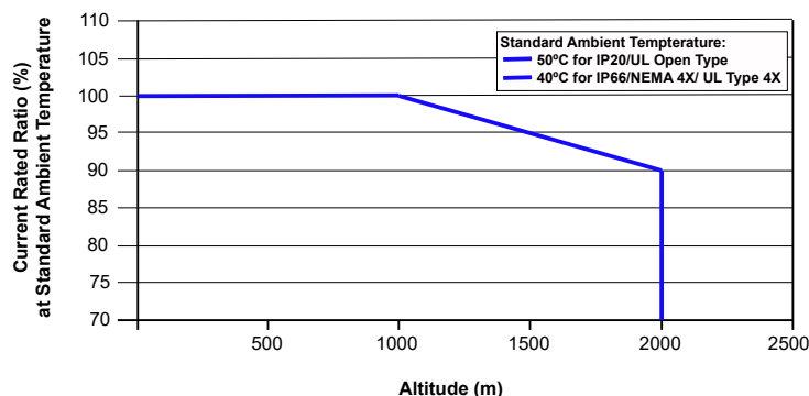
Derating for Altitude
