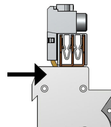
2- and 3-Phase Feeder Terminal
