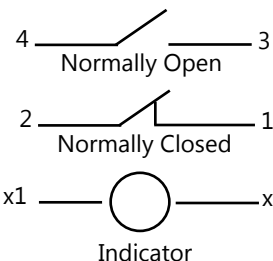
Typical Wiring
