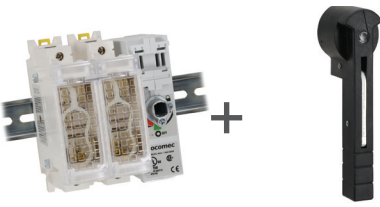
Switch Body
