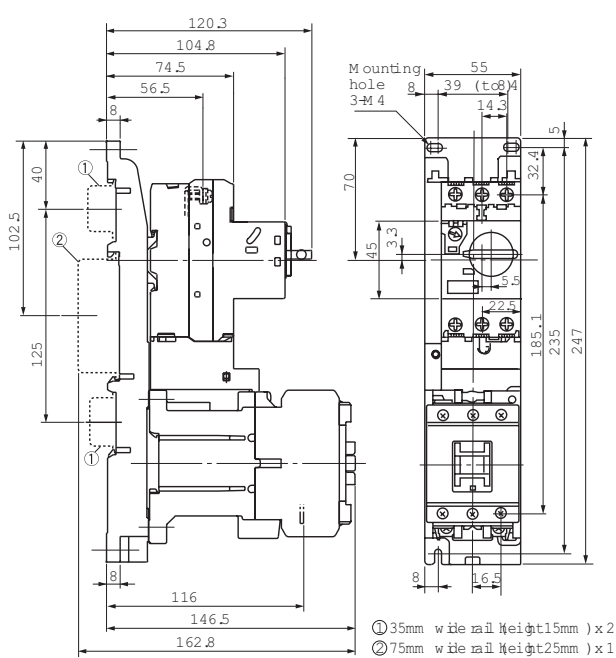
BM3RHB-xxx + SC-E1G-xxx
