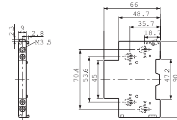
Auxiliary contacts side mounting BZ0WU AAL, BZ0WU ABL, BZ0WUBBL
