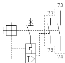
Auxiliary and alarm contact blocks BZ0WKU AA
