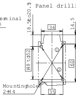
Panel drilling
