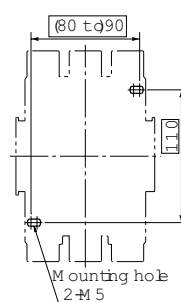
Panel drilling
