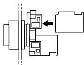
Snap-fitting of contact blocks
