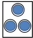
Rated current 800A 300 MCM x 3 37 strands each
