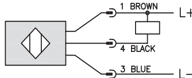
Diagram 2 NPN Output
