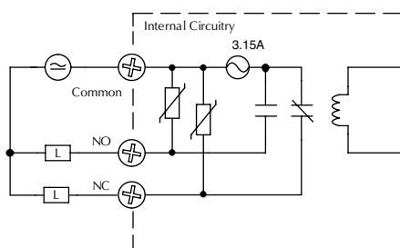
Typical Circuit
