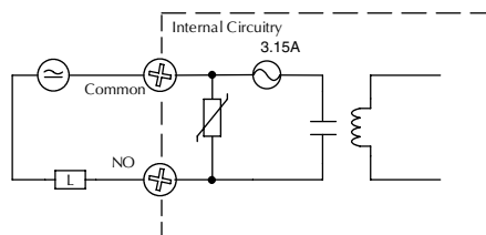
Typical Circuit
