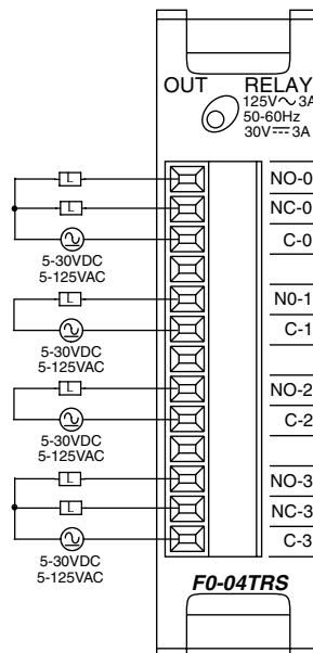
Typical Circuit
