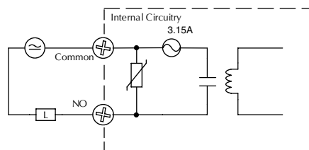
Typical Circuit
