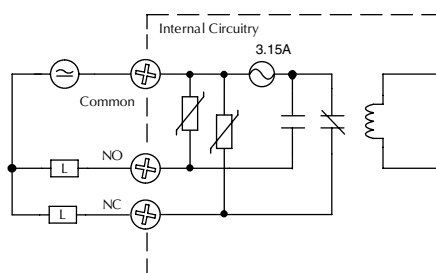
Typical Circuit
