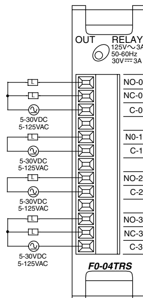
Typical Circuit
