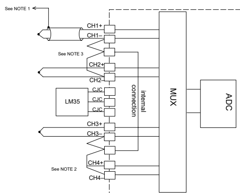
Thermocouple Input wiring diagram
