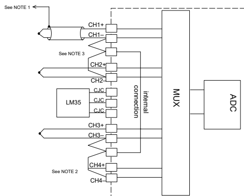
Thermocouple Input wiring diagram
