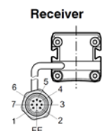
M12 pigtail, 0.3 m, 8 pins
