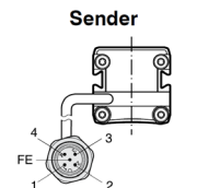
M12 pigtail, 0.3 m, 5 pins
