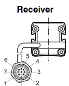
M12 pigtail, 0.3 m, 8 pins
