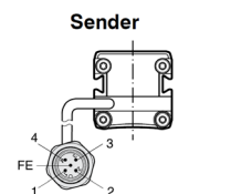
M12 pigtail, 0.3 m, 5 pins
