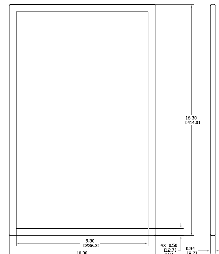
TA10-FILTER-3
