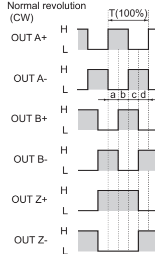
Line Driver Models (TRDA25RNxxxVWDxx)
