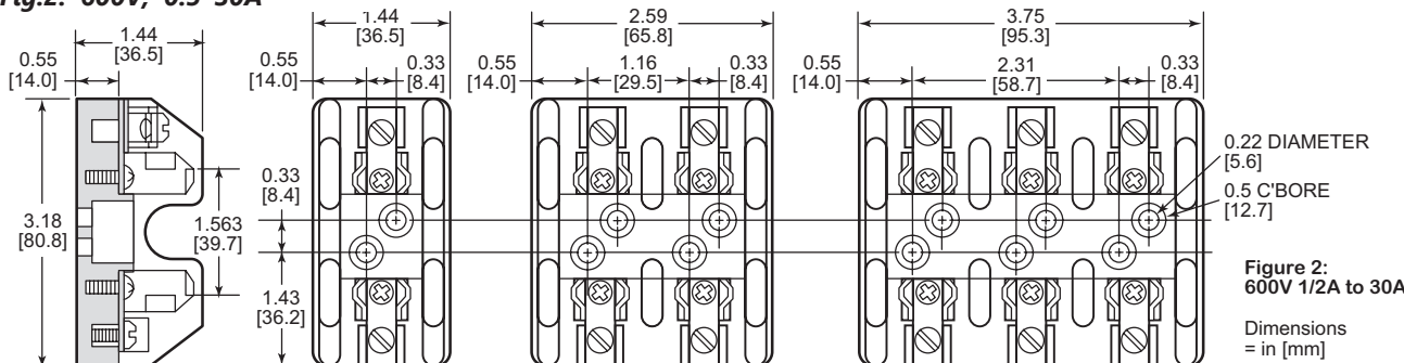
Fig.2: 600V; 0.5–30A
