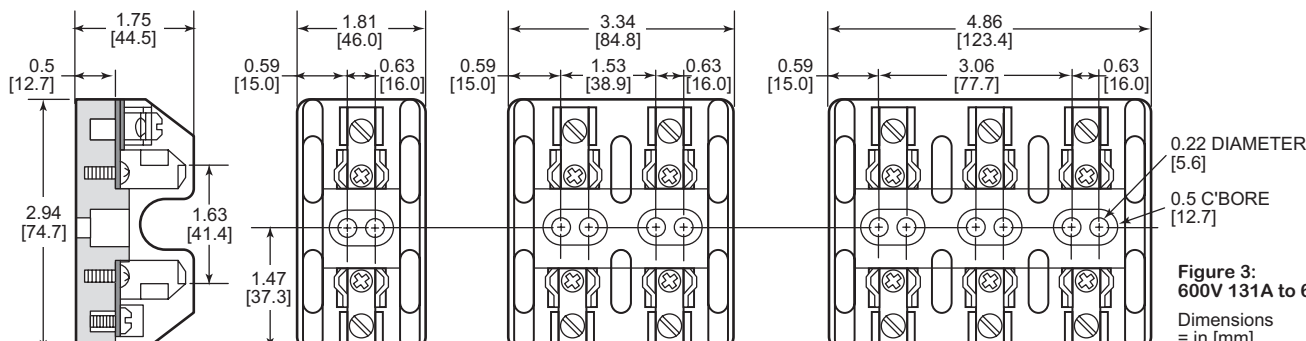
Fig.3: 600V; 31–60A
