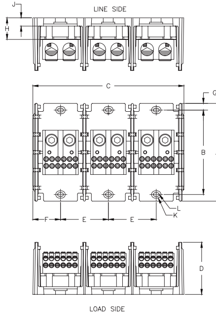
Optional Cover for PB3061, PB3062, PB3063 PB3121, PB3122, PB3123
