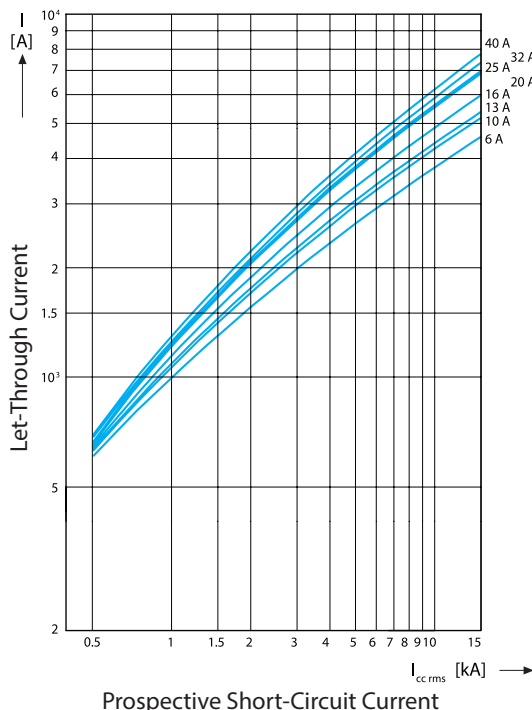
Let-through current I Characteristic D
