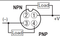
Diagram 4 4-wire PNP/NPN Output
