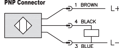
PNP Connector
