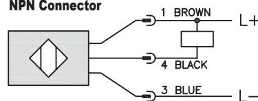
NPN Connector
