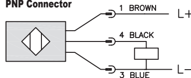
PNP Connector
