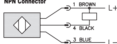
NPN Connector
