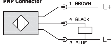
PNP Connector
